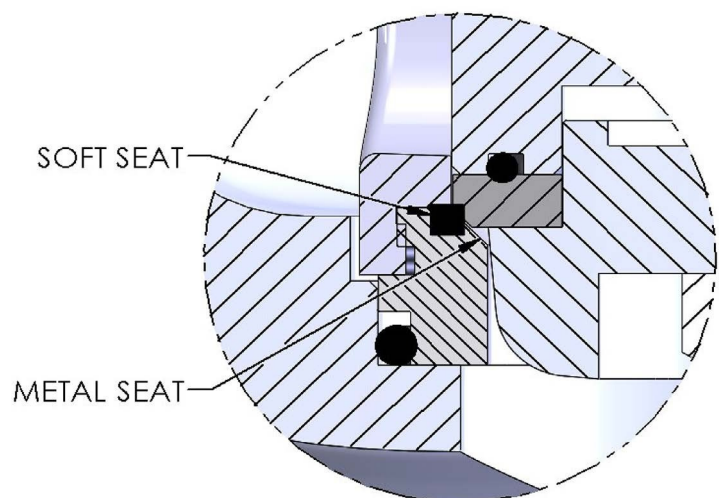
Seat Detail
